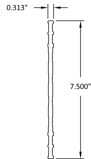
25 HINGE BACKER PLATE
