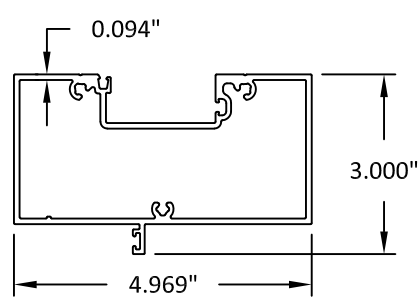
18 TRANSOM ADAPTOR (INS)
