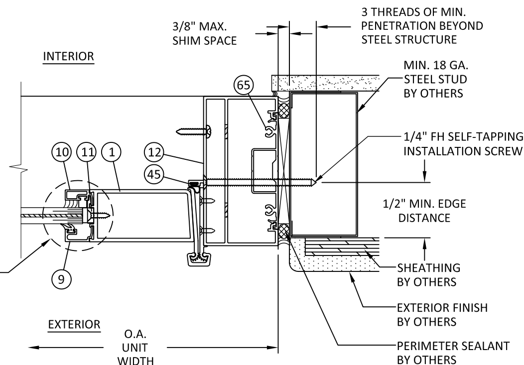
G HORIZONTAL SECTION 4 DOOR JAMB - STEEL STUD ROTON CONTINUOUS HINGE
