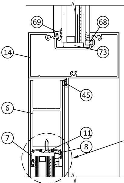
N 6 VERTICAL SECTION TRANSOM BAR
