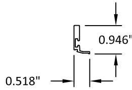
INT. GLASS STOP (1")
