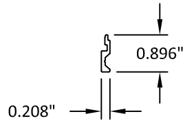
10" BOTTOM RAIL
