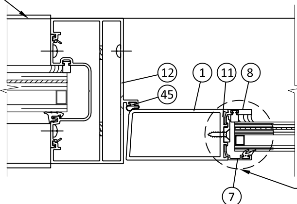
M 6 HORIZONTAL SECTION DOOR JAMB - STOREFRONT INSTALLATION
