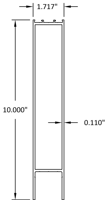
10" BOTTOM RAIL
