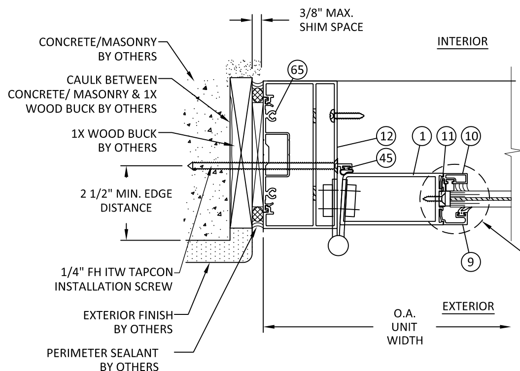
E HORIZONTAL SECTION 4 DOOR JAMB - CONCRETE/MASONRY STANDARD BUTT HINGE
