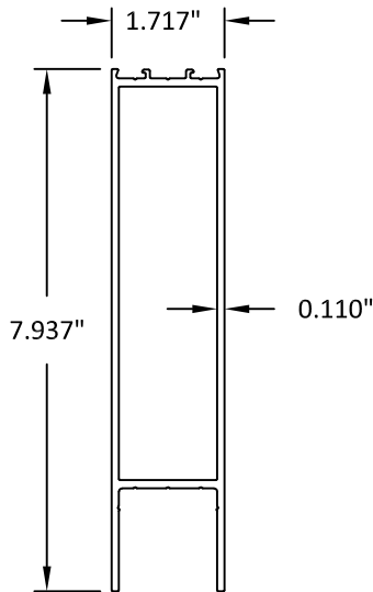
8" BOTTOM RAIL
