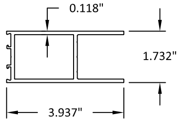
INT. GLASS STOP (9/16")
